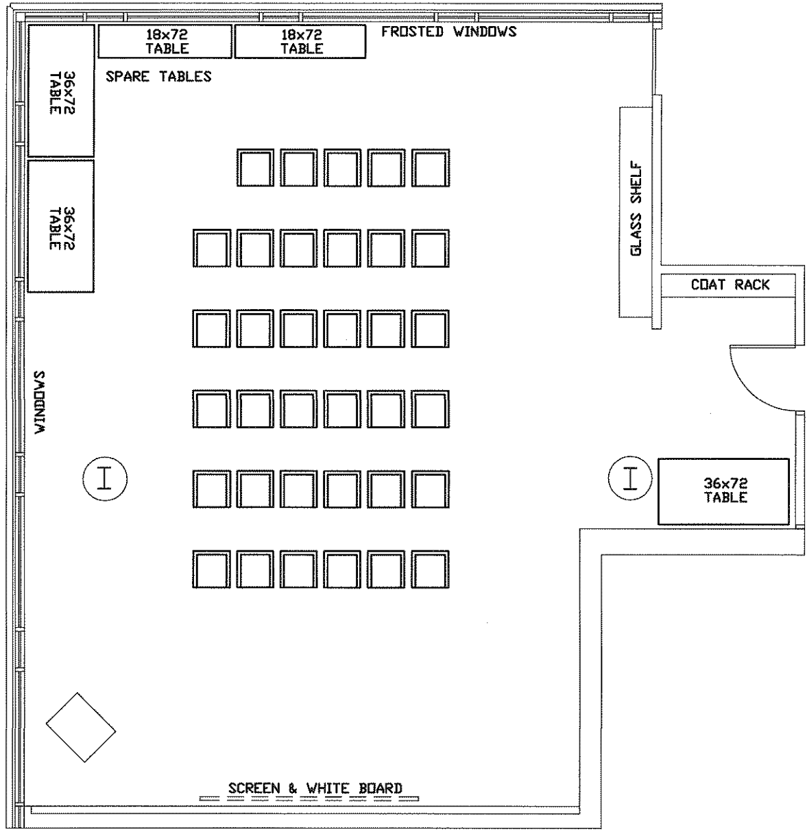
25' x 36' FORD ROOM THEATER LAYOUT
